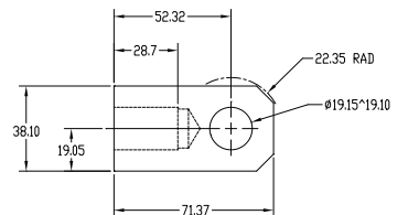
Female Eye Female Thread shown on drawings above.
